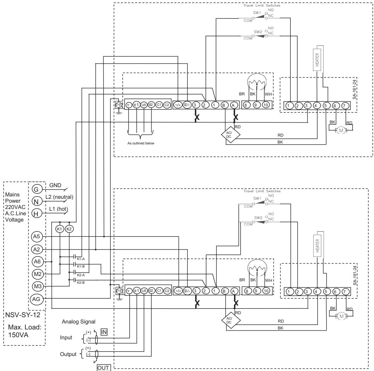
Wiring diagram for multiple proportional SY series 220 VAC actuators.
