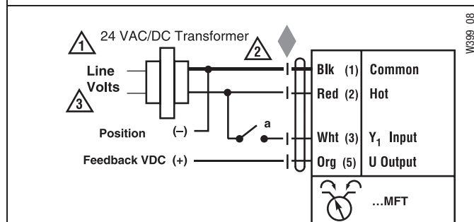
On/Off control
